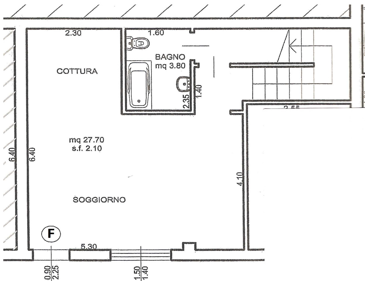
PIANO TERRA
